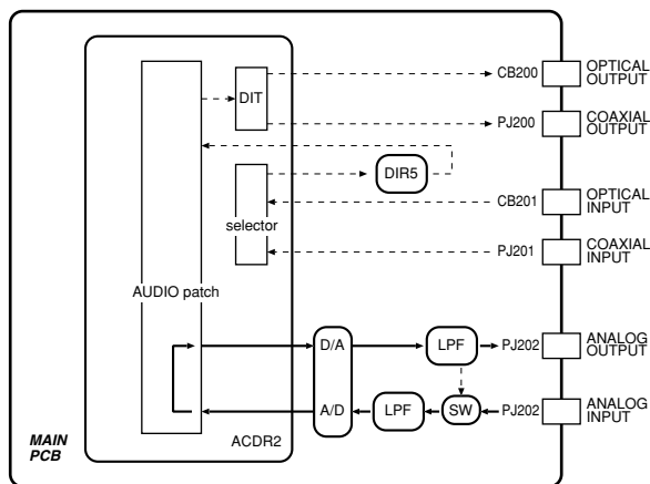
Signal flow diagram of Mode 2.
